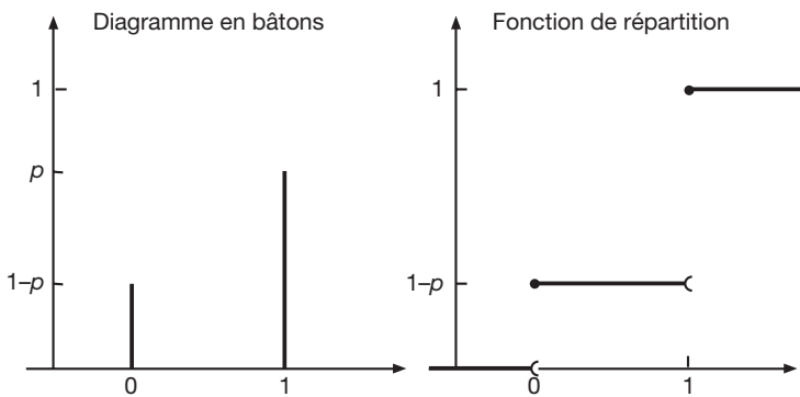
Figure 6.1 – Loi de Bernoulli
