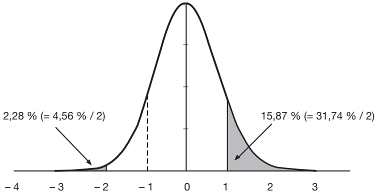
Figure 7.8 – Dispersion de la loi normale
